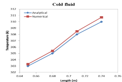
Figure.7. Temperature variation of cold body along the spiral plate heat exchanger
